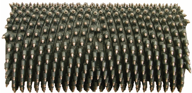
Fine cutting rotor with 6 mm tool spacing and welded tool holders.
