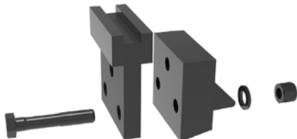
ABOVE: Exclusive 3-piece conical tool holders BELOW: Reversible, replaceable carbide-faced loading paddles
