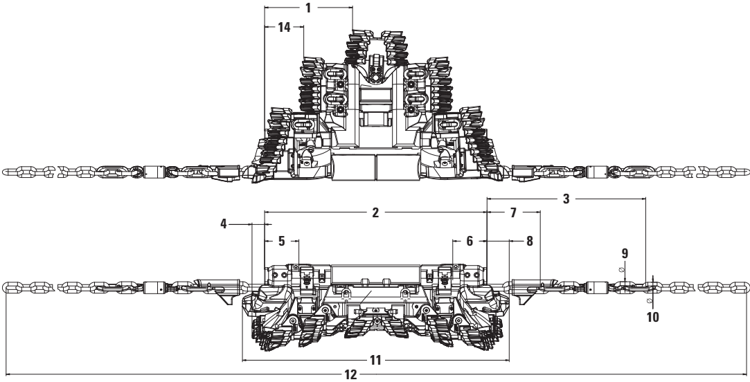
Dimensions – Plow Body Setup Option 3 (All dimensions are approximate.)
