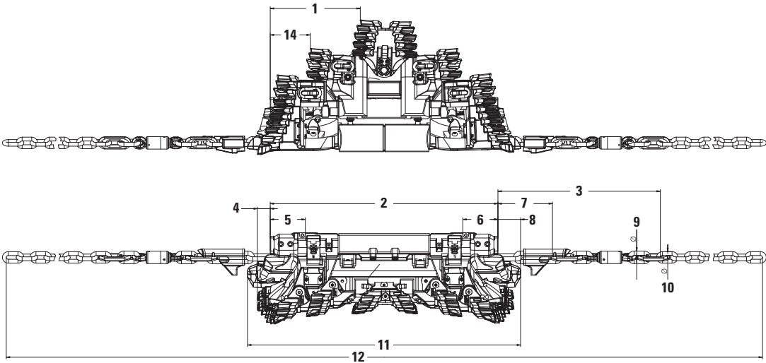
Dimensions – Plow Body Setup Option 2 (All dimensions are approximate.)
